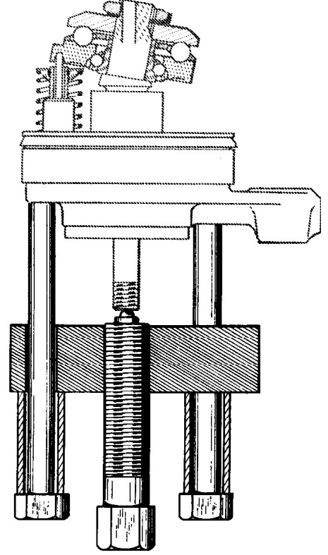
Fig. 3 EXTRACTION OF THE SHAFT
